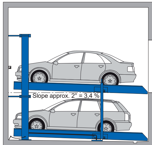
System lowered
