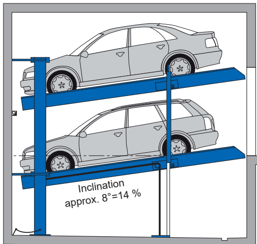
System raised
